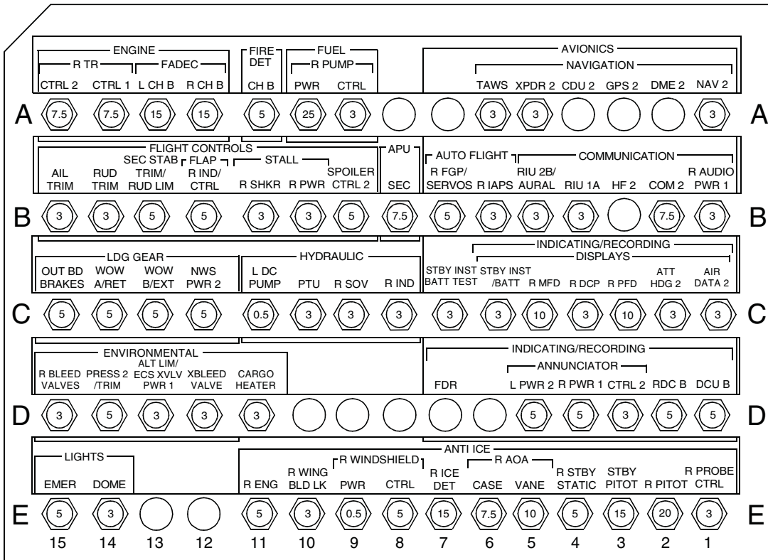
CB2 COPILOT CIRCUIT BREAKER PANEL (TYPICAL)
