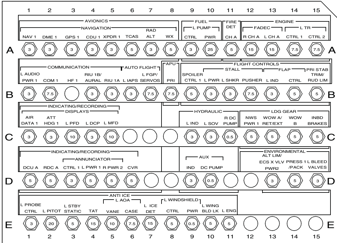
CB1 PILOT CIRCUIT BREAKER PANEL (TYPICAL)
