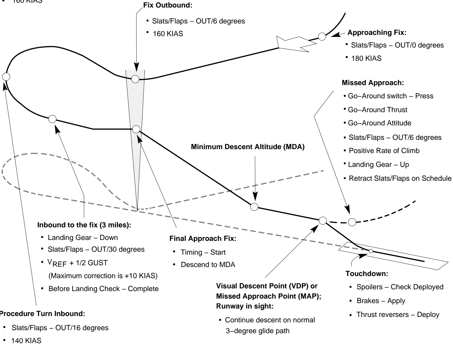
Non-Precision Approach Figure 04-08-2
