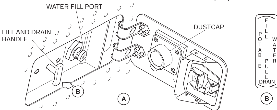
Potable Water Service and Drain Panel Lavatory Water System Figure 21-20-2
