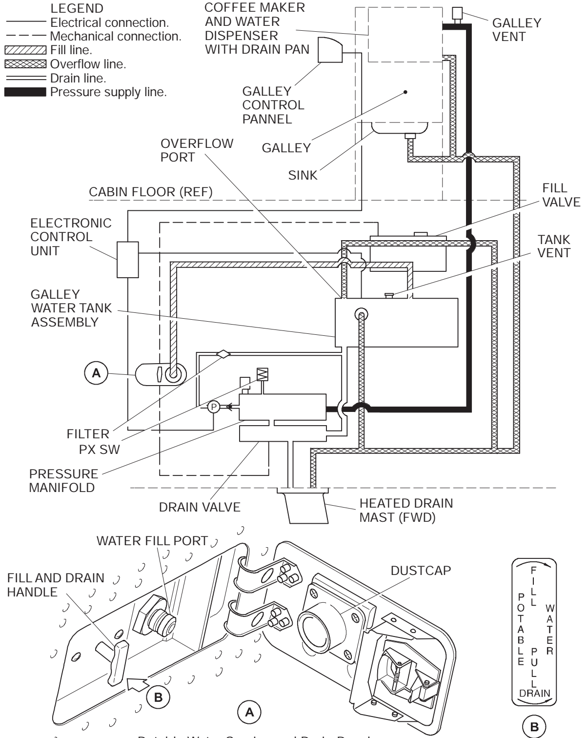
Potable Water Service and Drain Panel Galley Potable Water System Figure 21-20-1
