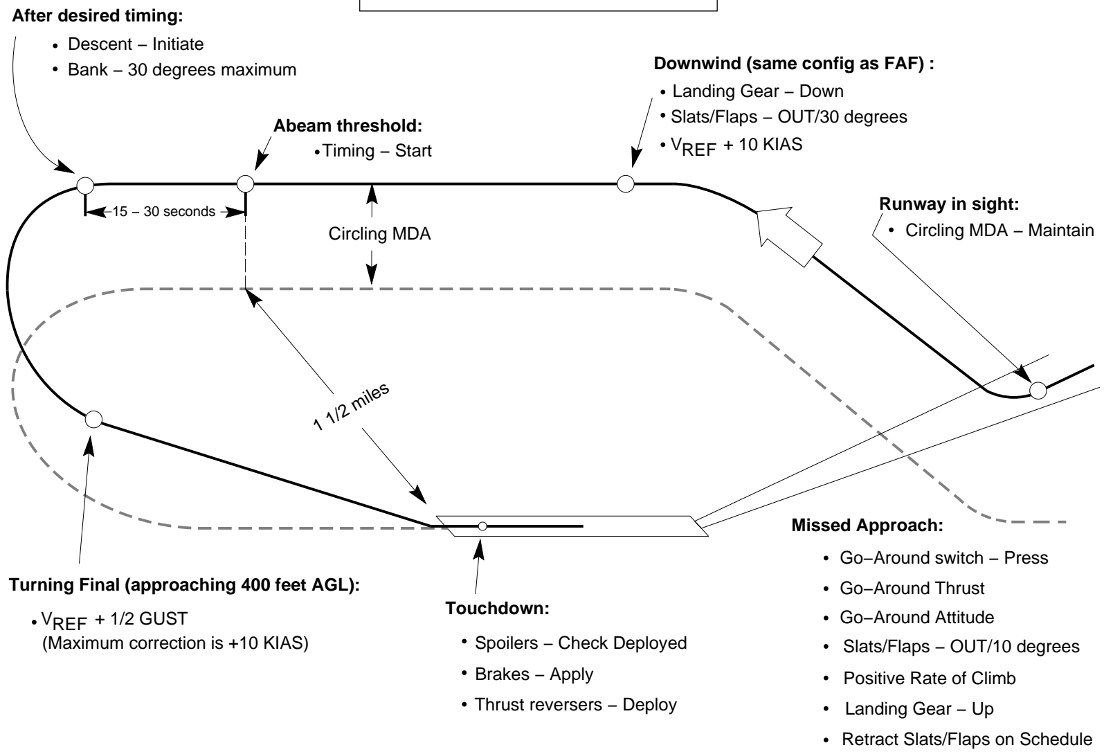
Circling Approach Figure 04-08-3
